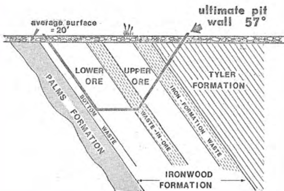
Penokee Range iron ore deposit and potential pit design. 10
